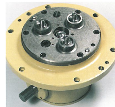
Left: Gearbox disassembled for rebuilding. Below: Refurbished to "like new" condition and ready for reinstallation.
